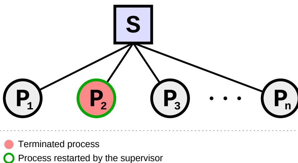
Figure 5.1: One_For_One Supervision
